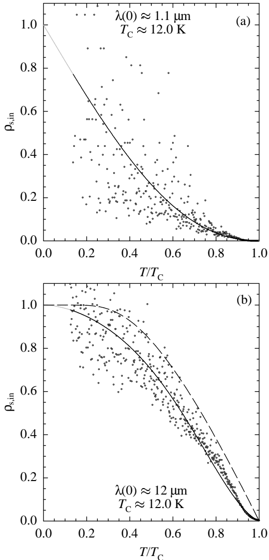
Fig. 1. In-plane superfluid density for (a) annealed and (b) quenched sample. The solid line is a fit to the d -wave expressions, and the dashed line presents the s -wave model.
