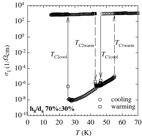
Figure 1. A typical conductivity versus temperature cycle below 100 K with two phase transitions in cooling and in warming half-cycle, obtained by dc conductivity measurements.
