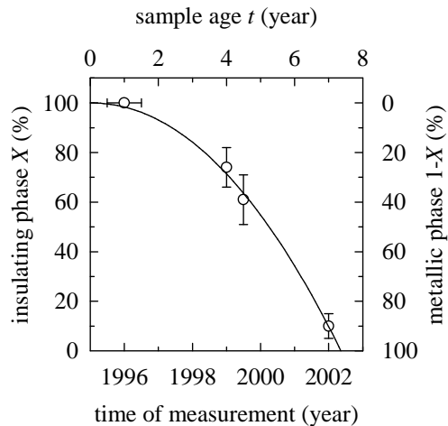
Figure 8. Percent of metallic phase ( 1 - X ) occurrences in the cooling half-cycle for “best”, well-defined, slow-cooling conditions as the function of the sample age. Full line is the fit to the power-law. The point with the horizontal error bar is based on the data obtained on fresh samples (see Text).
