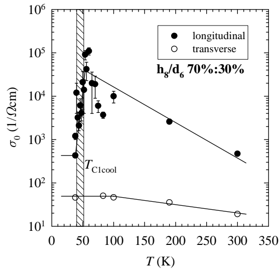
Figure 7. Longitudinal and transverse conductivity versus temperature, obtained by submillimetre quasioptical measurements. Shaded area represents the variation of T_{C1cool} among different samples. Full lines are guides for the eye.
