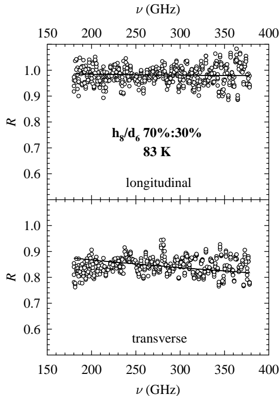
Figure 5. Reflectivity versus frequency for longitudinally and transversely polarized radiation above the phase transition range at 83 K. Full lines are fits to Hagen-Rubens expression (see Text).
