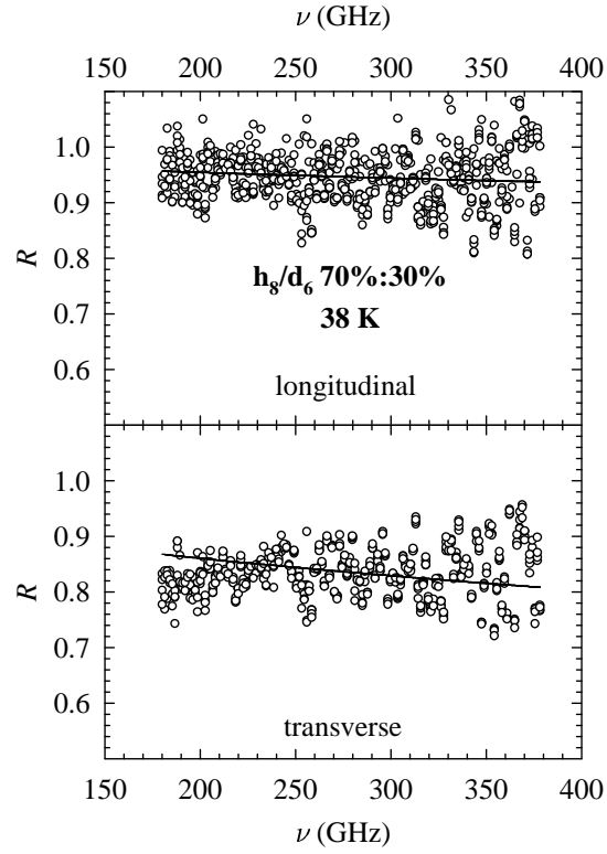
Figure 6. Reflectivity versus frequency for longitudinally and transversely polarized radiation below the phase transition range at 38 K. Full lines are fits to Hagen-Rubens expression. (see Text)
