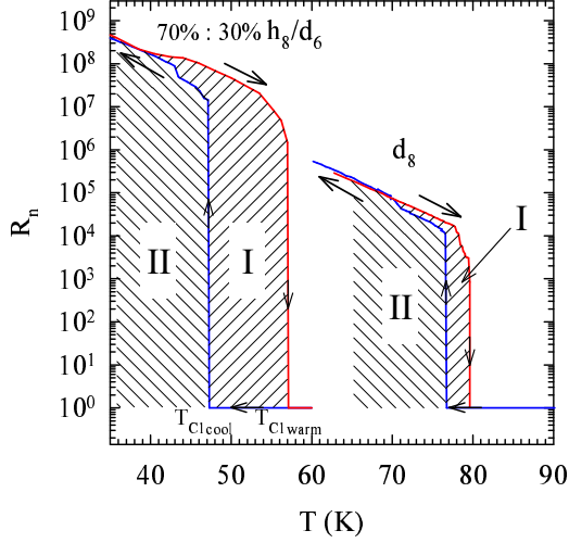
Fig. 1. Temperature dependence of the normalized resistance ( R_n = R(T)/R(100 \text{ K}) , where 1/R(100 \text{ K}) corresponds to a conductivity of about 1000 \text{ Scm}^{-1} ) in the cooling and warming cycle of the h_8/d_6 70%:30% system and the d_8 system.
