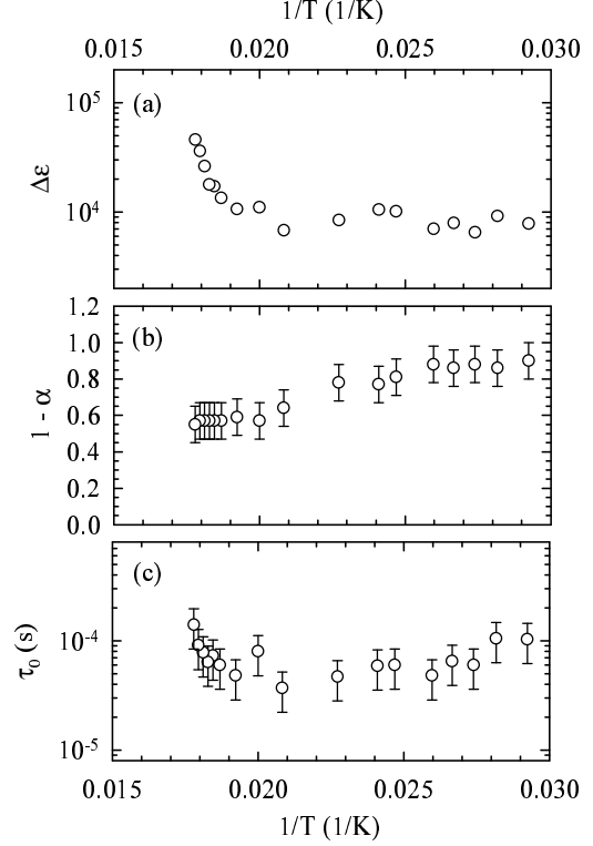
Fig. 6. (a) Relaxation strength ( \Delta\varepsilon ), (b) shape parameter ( 1-\alpha ) and (c) mean relaxation time ( \tau_0 ) versus inverse temperature in the h_8/d_6 70%:30% system.
