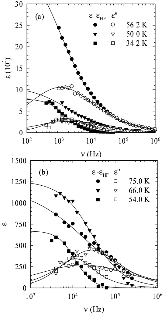
Fig. 3. Frequency dependence (log scale) of the real and imaginary parts of the dielectric function at three selected temperatures for (a) the h_8/d_6 70%:30% system and for (b) the d_8 system. Full lines are fits to the HN form.
