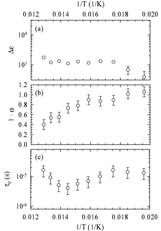
Fig. 7. (a) Relaxation strength ( \Delta\varepsilon ), (b) shape parameter ( 1-\alpha ) and (c) mean relaxation time ( \tau_0 ) versus inverse temperature in the d_8 system.
